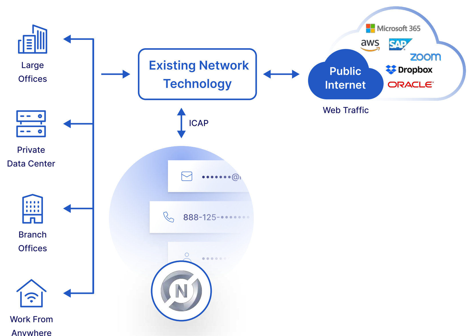
Figure 1: Nullafi Shield sits between applications and endpoints and simply “ties in” with existing network technology to obfuscate individual data elements according to the user's identity, before they get to the user's device.
